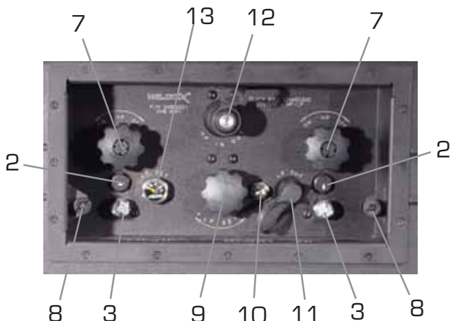
HP/LP Quick-Fill Charging System Control Panel
