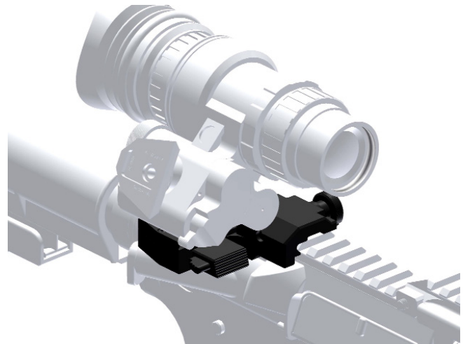
The AN/PVS-18 NVG Weapon Mount Attached to the Top Rail of the M4-A1, Affixed to the AN/PVS-18
