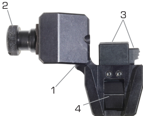
AN/PVS-18 NVG Weapon Mount
