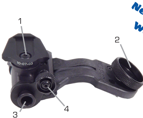
AN/PVS-14 Arm with NVG Interface Shoe (Oriented for Left Eye Operation)
