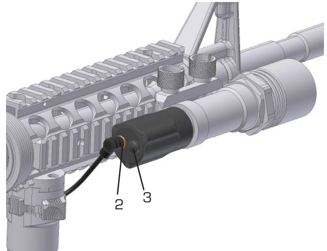
The Wilcox Multi-Function Tail Cap Switch (P/N 44700G02) Mounted to the SureFire WeaponLight (Illustrated with the M-4 Weapon and Wilcox TCVG)
